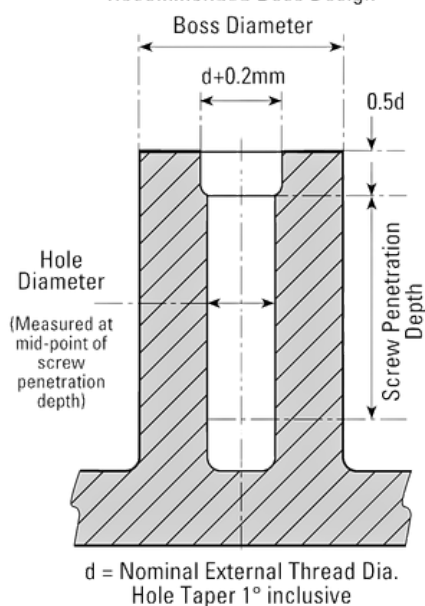
Recommended Boss Design
