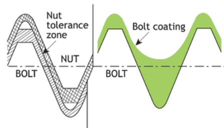
The Pre-Applied Thread Sealant Principle
