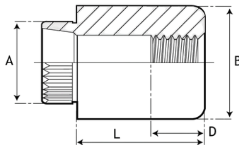
Product Code ARBSO
