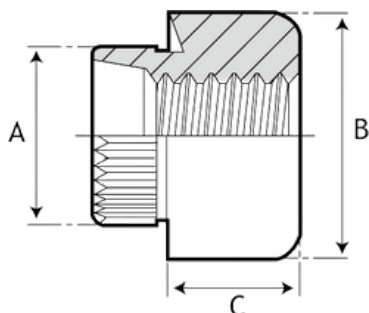
Product Code ARB
