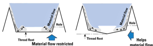
Fiat Root thread v PT Profied Root thread
