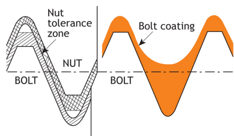
Micro Encapsulated Adhesive Principle
