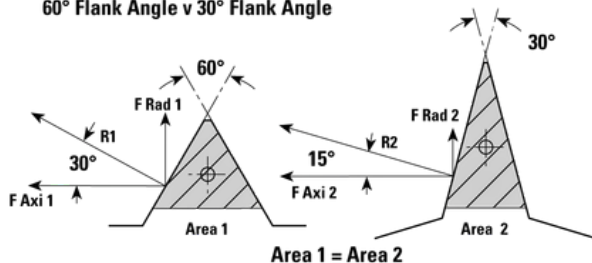
60° Flank Angle v 30° Flank Angle
