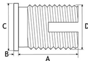
PRODUCT CODE [ HSCT ]
