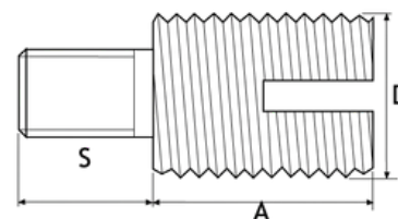
PRODUCT CODE [ SCTS ]
