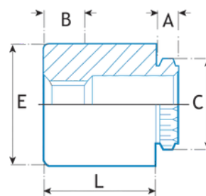
PRODUCT CODE SCBR
